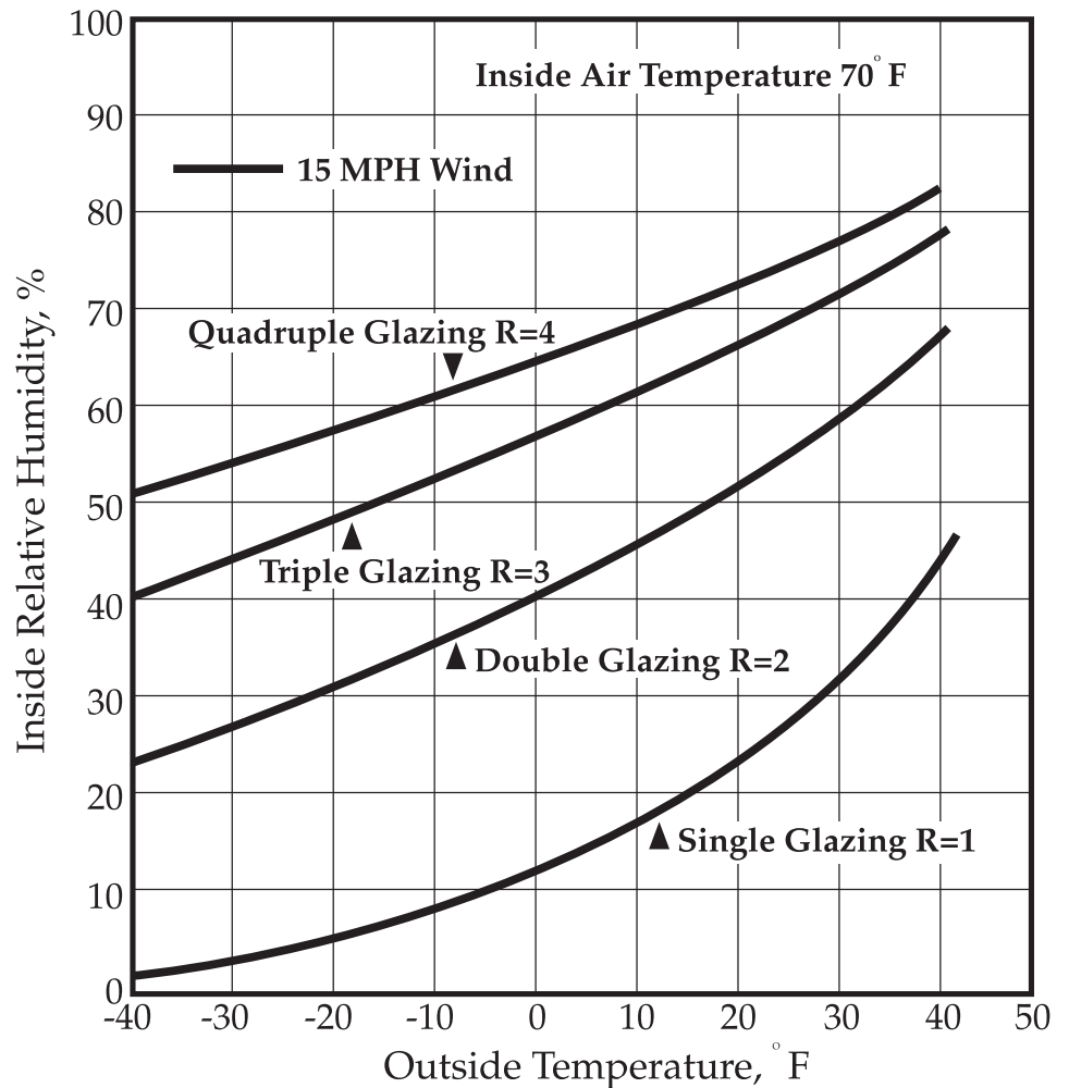
Figure 2. Condensation on window surfaces as affected by outside temperature, inside relative humidity and window type.
