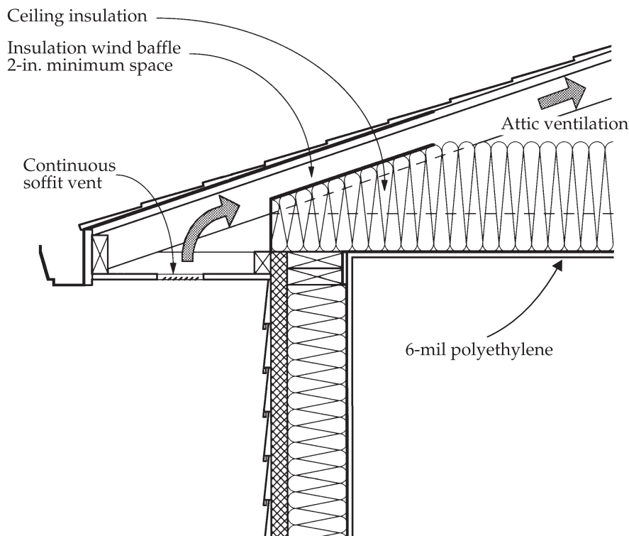
Figure 4. Air enters for attic ventilation at the eave and exhausts near the roof peak.
